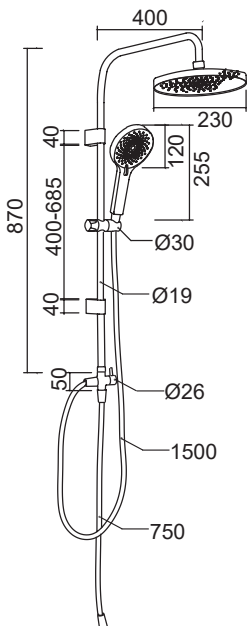
Brass Diverter
