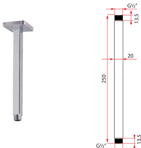
RSA-VAS-250
